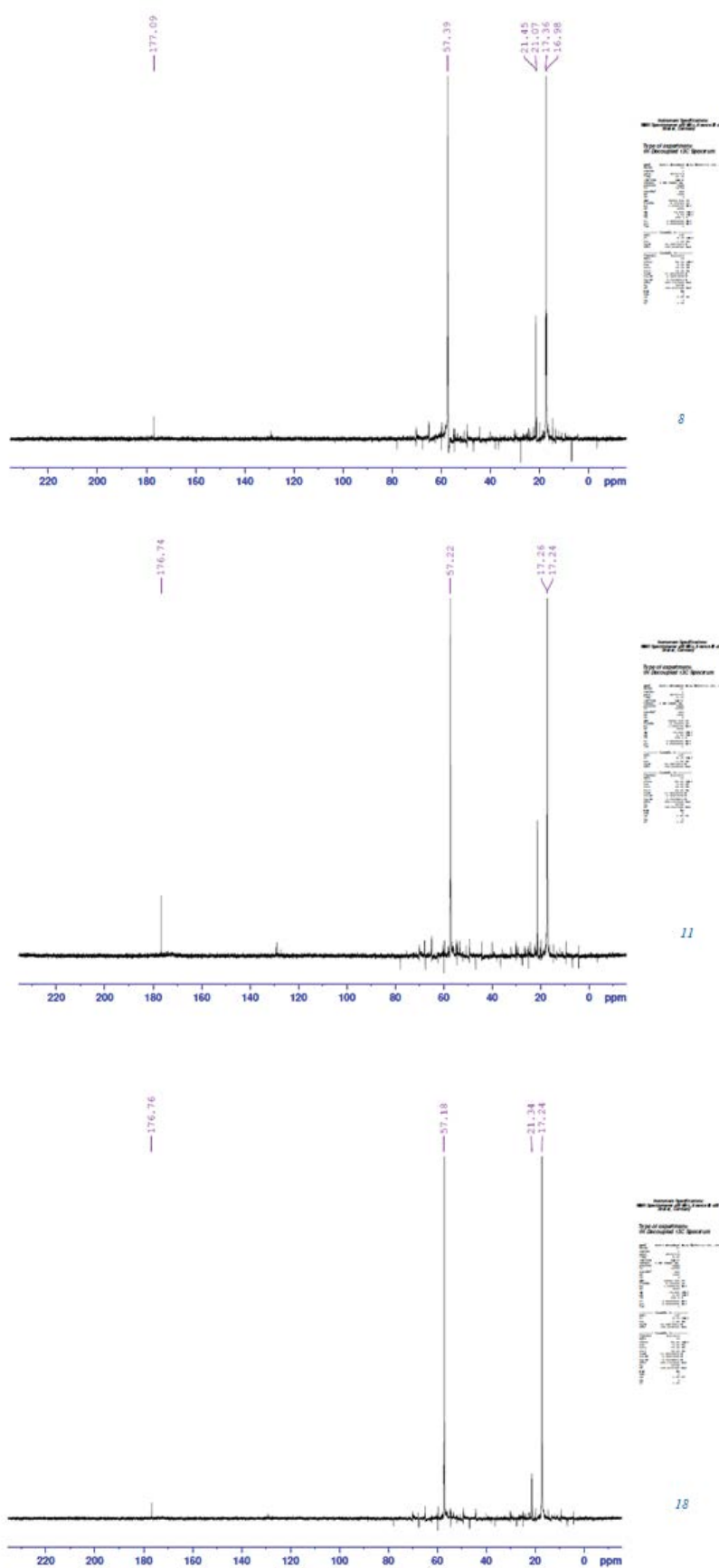
Figure 3. 13 C NMR (300 MHz) spectrum of the bioactive metabolites produced by Streptomyces isolates.
